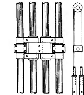
⑤ Cable network attachment
